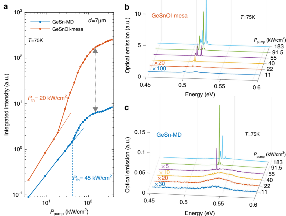
Fig. 3 GeSnOI mesa versus as-grown GeSn microdisk laser. a Light-Light (L-L) curves of 7 μm diameter GeSn microdisks and GeSnOI mesas with 360-nm-thick GeSn at 75 K under pulsed pumping ( b ) and c PL spectra at 75 K for various pulsed excitation powers for the GeSnOI mesa and the GeSn-MD, respectively. Excitation levels are given by the peak power densities
