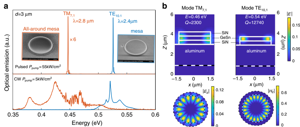
Fig. 6 Tensile strain tuning of GeSnOI laser emission. a Spectra below and above threshold density for 3 \mu\text{m} diameter GeSnOI mesas with (red curves) or without (blue curves) top SiN stressors. In both cases, the active GeSn layer thickness was 400 nm. b Simulated optical fields and theoretical Q -factor values of \text{TM}_{7,1} and \text{TE}_{10,1} lasing modes for a tensile-strained GeSnOI mesa with a SiN stressor on top and a quasi-relaxed GeSnOI mesa without the top SiN stressor, respectively. Calculations have been performed with an aperiodic Fourier modal method dedicated to body-of-revolution objects 45
