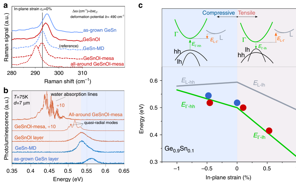
Fig. 2 Optical analysis of strain. a Raman spectra of LO-phonon vibrations in the blanket, as-grown GeSn 10.5% on Ge SRB stacks, blanket GeSnOI stacks, GeSn-on-Ge SRB microdisks, GeSnOI mesas, and all-around GeSnOI mesas. The diameter of disks and mesa was 7 \mu\text{m} . b Photoluminescence spectra of GeSn layers as in (a) excited with cw optical pumping. c Direct and indirect bandgap energies of GeSn as a function of strain. Direct bandgap energies from PL measurements appear as blue circles for the as-grown GeSn 10.5% on Ge SRB stack and the GeSn-on-Ge SRB microdisks. Red circles show the PL energies for the blanket GeSnOI stack, the GeSnOI mesa, and the all-around GeSnOI mesa (from left to right). Full lines are calculated direct bandgap (green) and indirect bandgap (gray) energies as functions of strain using model as described in ref. 5 . The top picture is a schematic scenario of band structure for compressive and tensile-strained GeSn
