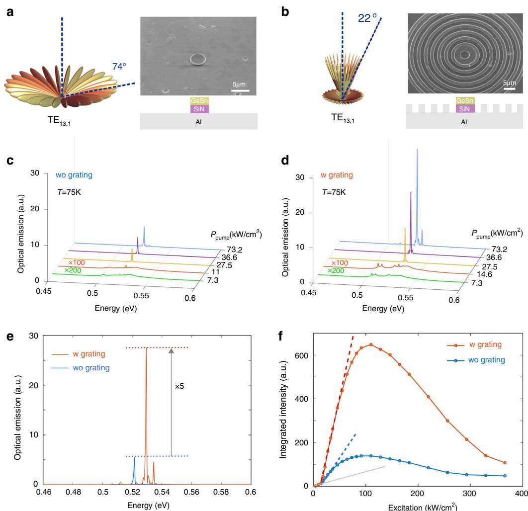
Fig. 7 Vertical out-coupling of GeSnOI mesa lasing WGM. a, b SEM images and calculated emission patterns of 4 \mu\text{m} diameter GeSnOI mesas without and with Al circular grating (7 rings spaced by 3 \mu\text{m} with a duty cycle of 50%). Calculations have been performed with an aperiodic Fourier modal method dedicated to body-of-revolution objects 45 . c, d Power-dependent spectra without and with Al circular grating. e Spectra with and without grating for a 73.2 \text{kW}/\text{cm}^2 excitation density. f L–L curves of GeSnOI lasers with and without grating
