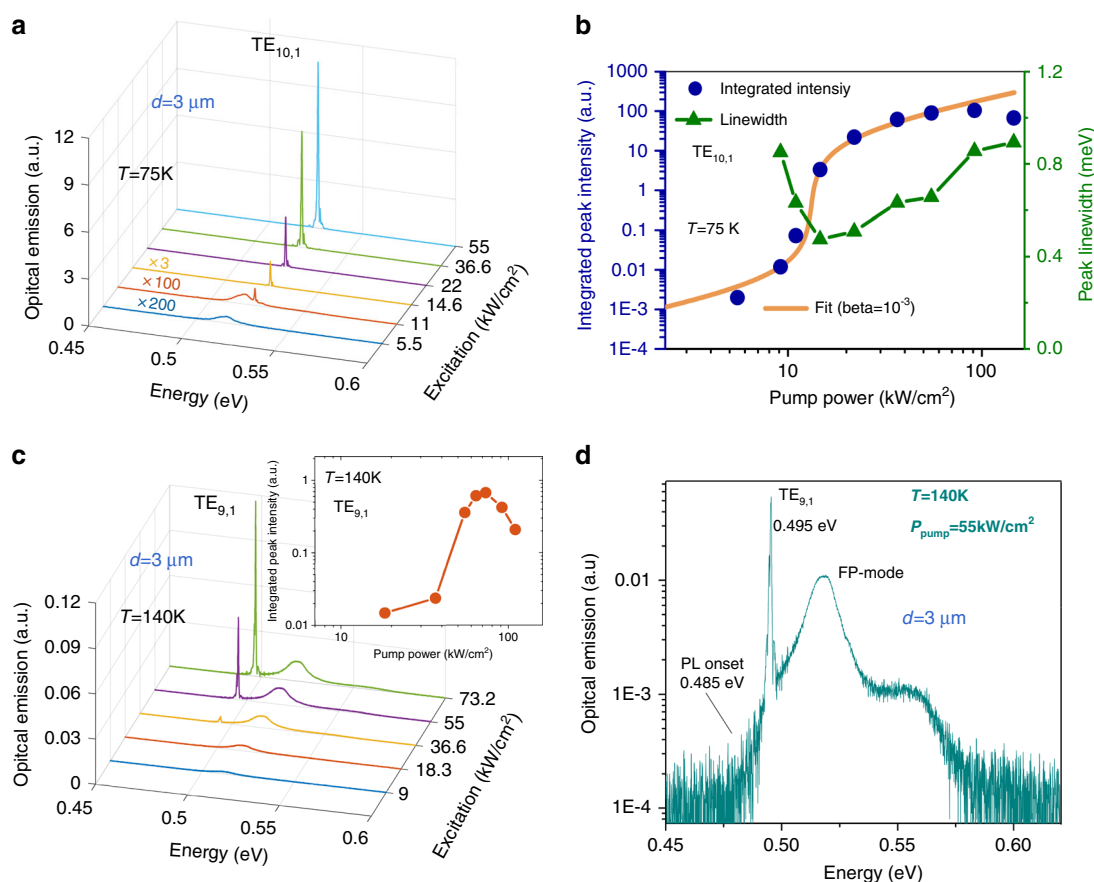
Fig. 5 Down-scaled GeSnOI mesa laser. a Pulsed PL spectra of 3 \mu\text{m} diameter GeSnOI mesa with 360-nm-thick GeSn under various excitation densities at 75 K. b the L-L curve of the laser mode \text{TE}_{10,1} at 75 K in log-log scale and mode linewidth as a function of the pump power. c same as a at 140 K, the inset shows the L-L curve in a log-log scale for the lasing mode which is the \text{TE}_{9,1} in this case. d Emission spectrum above threshold at 140 K highlighting the \text{TE}_{9,1} lasing mode position with respect to the spontaneous emission. The spontaneous emission is itself strongly modulated by broad peak that stems from Fabry-Pérot (FP) resonance. These FP-modes emit more favorably out-of-plane and are thus better collected than the WGMS
